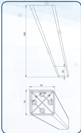
MANGO (70x70X200) mm 111353101121461 Ağaç -Krom
