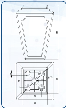
TAFLAN (60X60X130) mm 111122401140962 Beyaz
